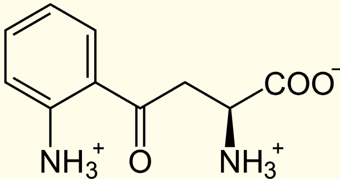
Kynurenin
